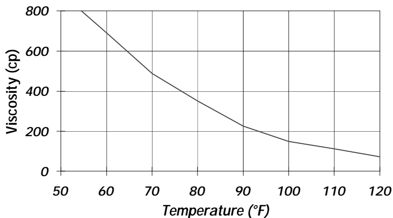
Viscosity vs. Temperature
