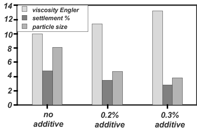
Figure 1. Effect of Redicote AP on the Properties of a CRS-1 Emulsion
